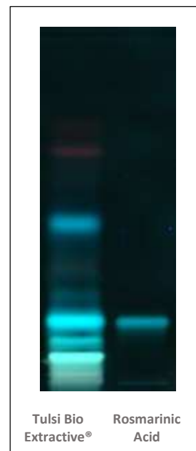
Figure 2. HPTLC Tannins of Tulsi Bio Extractive®
