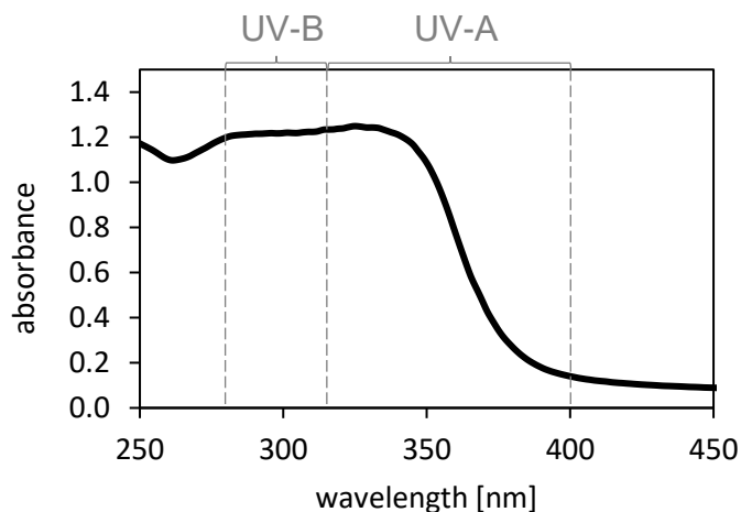
Figure 4. UV absorbance spectrum of 0.2% Tulsi Bio Extractive ®
